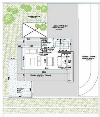
PLANTA BAJA / GROUND FLOOR
